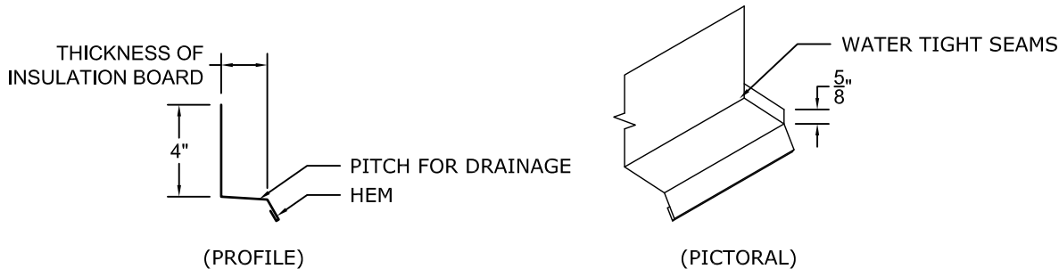
METAL HEAD FLASHING PROFILE
