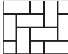
AS5 Herringbone Brick 3-3/4 x 8 x 1/2" mortar joint
